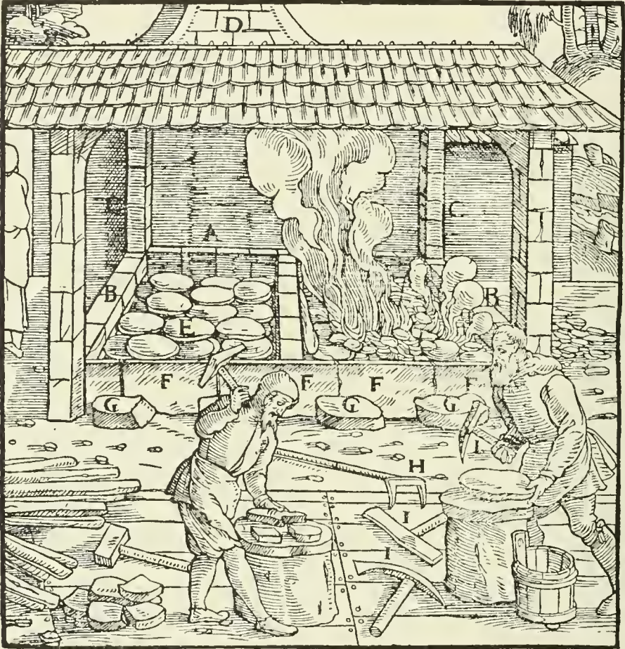
A—BACK WALL. B—WALLS AT THE SIDES. C—UPRIGHT POSTS. D—CHIMNEY. E—THE CAKES ARRANGED. F—IRON PLATES. G—ROCKS. H—RABBLE WITH TWO PRONGS. I—HAMMERS.
